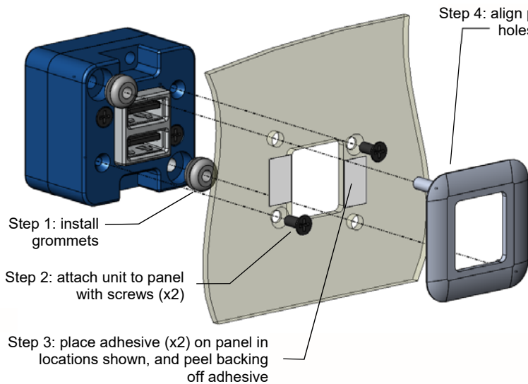
Figure 3.7 Rear Mount Installation with Cover
