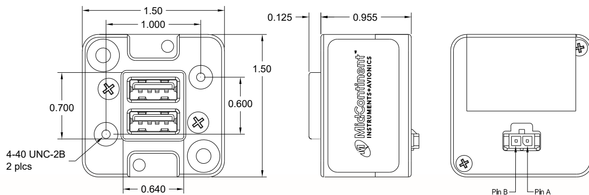
Figure 3.2 TA102 Outline Drawing
