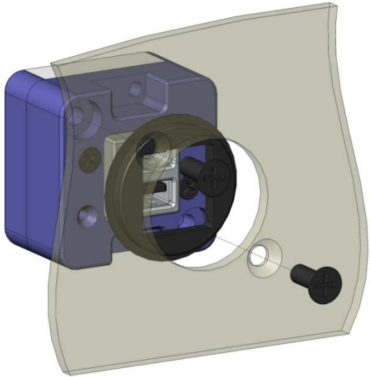
Figure 3.4 Circular Rear Mount Installation
