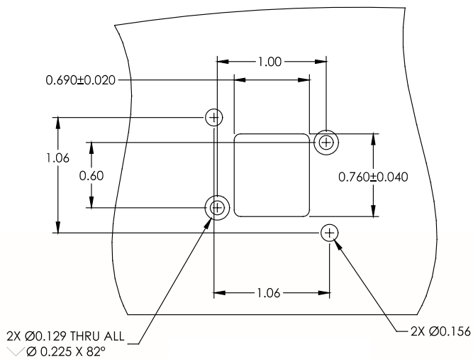
Panel Cutout Detail
